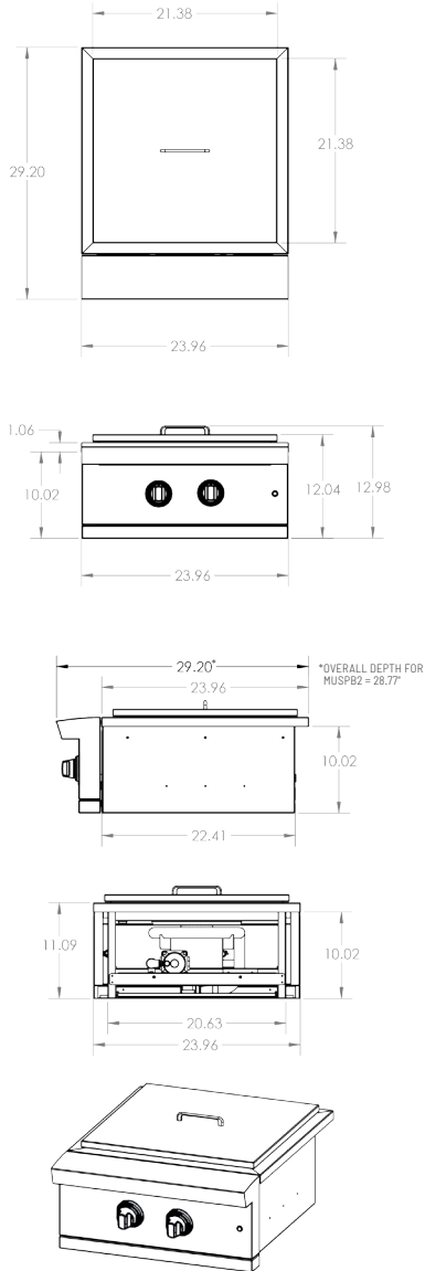
LINE DRAWING FOR ENCPB2, MUSPB2, ESTPB2 (ENCPB2 PICTURED)
