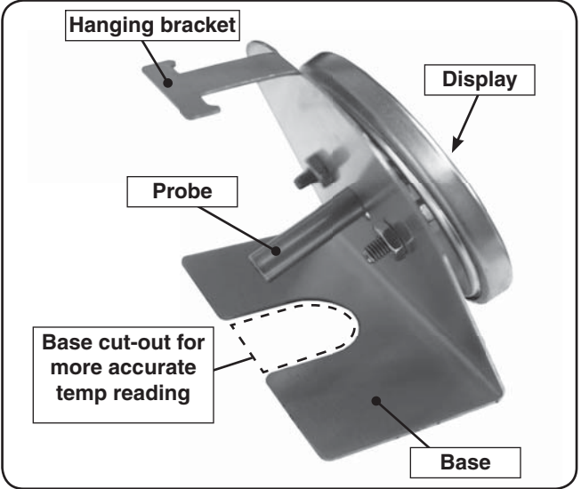
Fig. 1-2 Thermometer features
