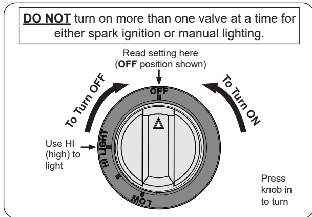
Fig. 33-1 Control knob
