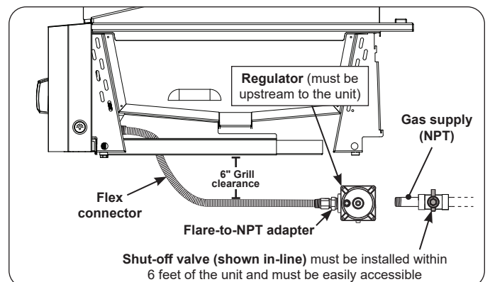
Fig. 28-4 Connecting to a gas line
