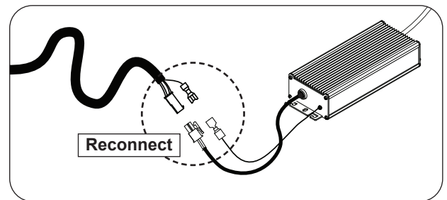
Fig. 28-2 Reconnect harness
