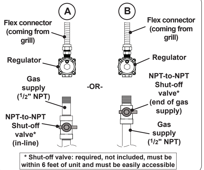
Fig. 28-3 Household propane & natural gas diagram
